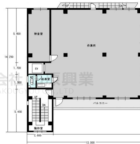
2F: 139.94㎡ (約42.33坪)
